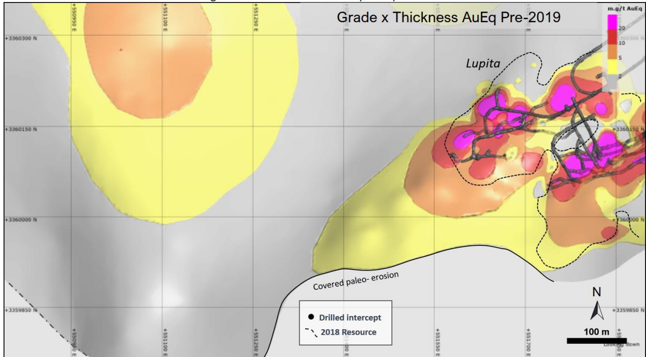
Figure 1 – Grade x Thickness Map of Lupita Area
